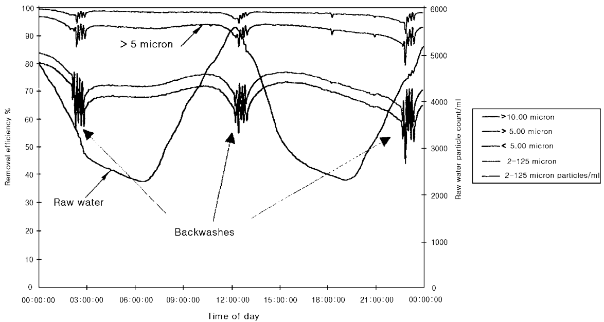
Average particle removal on the Atkins Fulford Microfilters at Burpham WSW, 01/06/97. Flow through plant = 19MI/day, number of filters on line = 8.
