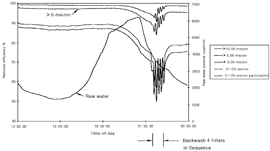
Average particle removal on the Atkins Fulford Microfilters at Burpham WSW, 28/05/97. Flow through plant = 19MI/day, number of filters on line = 9.
