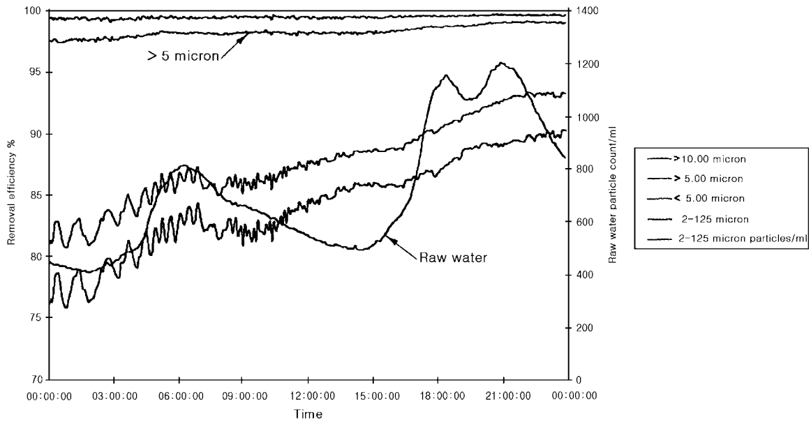
Average particle removal on the Atkins Fulford Microfilters at Burpham WSW, 29/04/97.
